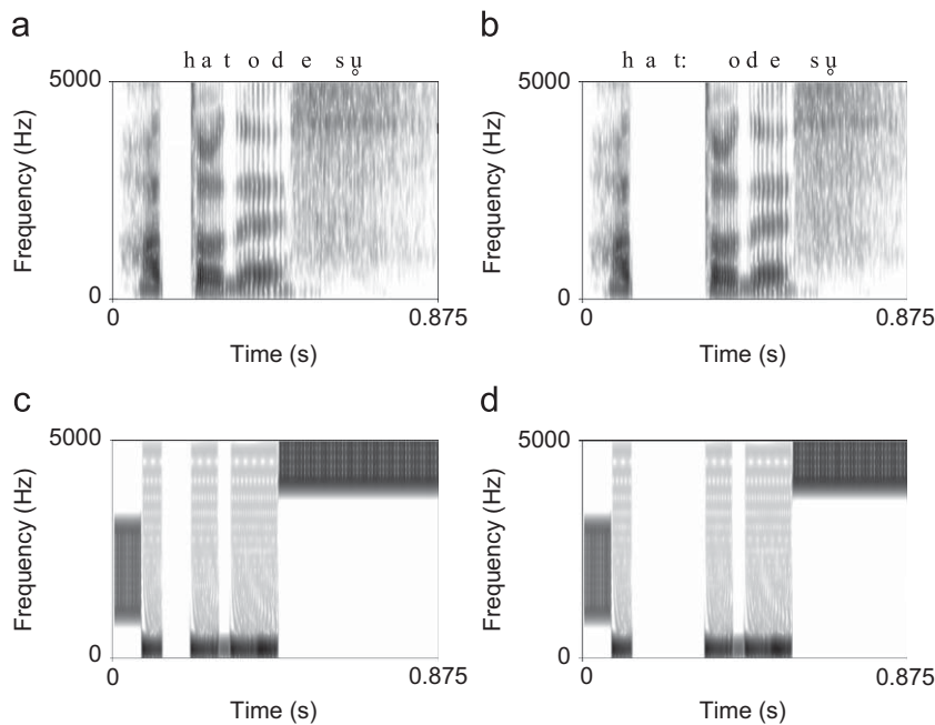
Fig. 1. Spectrograms of (a) a speech stimulus, [hato desu], with a short closure, (b) a long closure, and (c, d) corresponding non-speech analogues. The [esj] intervals are shorter in the (b, d) than (a, c) to make up for the increase in the duration of the silent interval.
