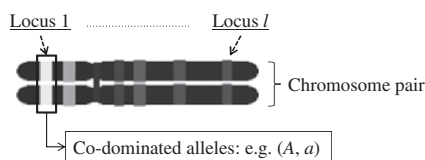
Fig. 1. An illustration of a chromosome pair with several loci from a diploid individual. Genotype is co-dominated by a pair of alleles at each locus.
