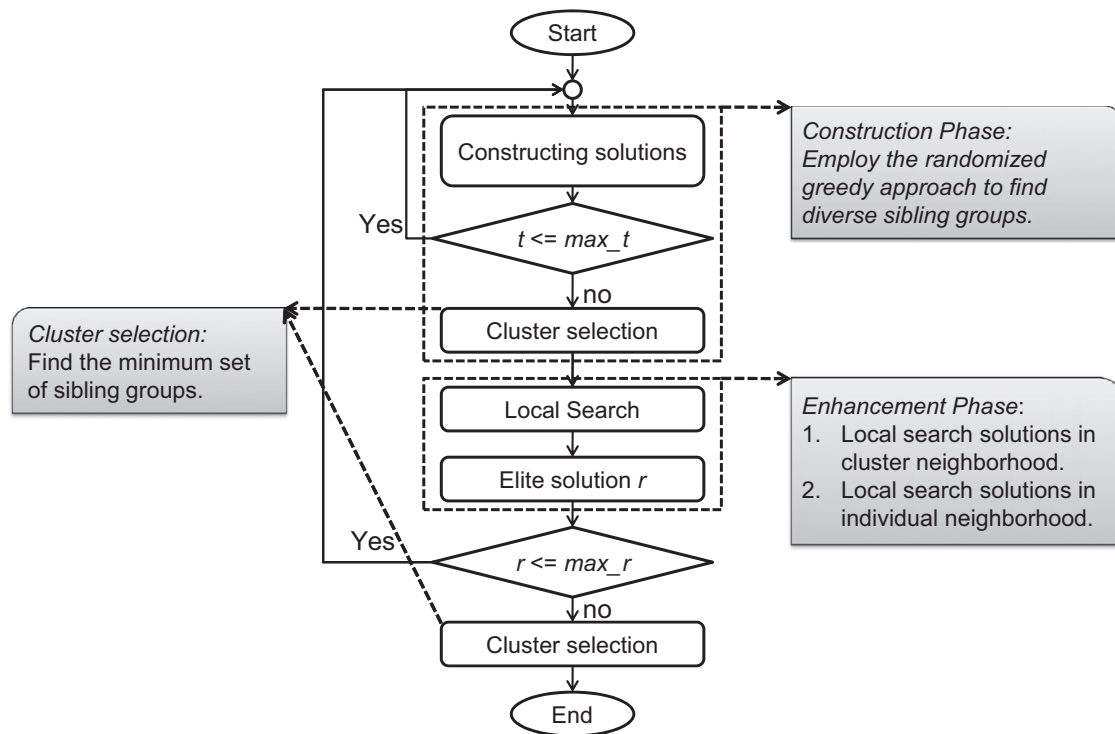
Fig. 3. Flow diagram of randomized greedy optimization algorithm. Construction phase is to construct a set of sibling groups with the randomized perturbations. Enhancement phase is to employ the two-stage local search to improve the solution quality. Cluster selection is to solve a set covering problem (SCP) to obtain the minimum set of sibling groups. A solution is defined as a set of sibling groups (clusters).
