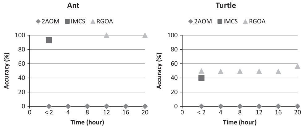
Fig. 4. Averaged accuracies of RGOA on real data sets (ant and turtle) are obtained over time shift, compared to 2AOM and IMCS approaches of Chaovalitwongse et al. [17]. Accuracy = 0 represents that no feasible solution is available by 2AOM at the time. For IMCS, all solutions are obtained within 2 h.
