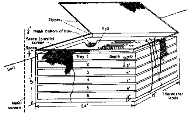
FIG. 2. Underground field cages used to study vertical Plethodon distribution under semi-natural conditions.
