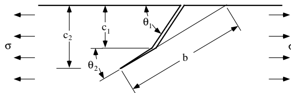
Fig. 10. A kinked edge crack in a half-plane under remote uniaxial tension.
