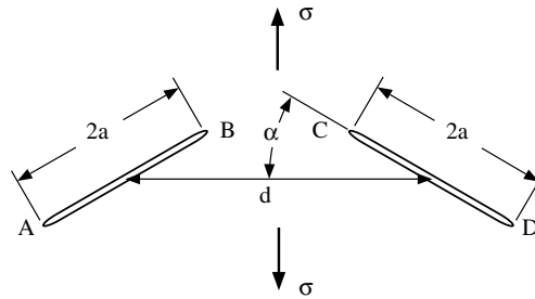
Fig. 8. Two inclined cracks under remote uniaxial tension.
