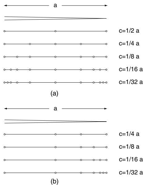
Fig. 3. (a) Symmetric and (b) asymmetrical crack elements for an edge crack.
